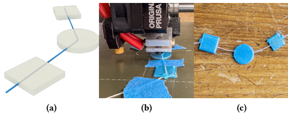
Figure 10: (a) A design for embedding cotton string via the manual printing process. (b) Using tape to secure the string; an anchor has just been printed via the “blob” technique, Section 5.4.4. (c) The resulting beaded string.
