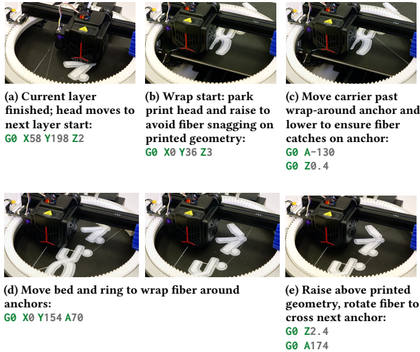
Figure 12: Wrap-around anchoring procedure as used in the “grabber” example (Section 6.7).
