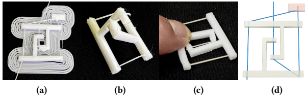
Figure 21: (a) A pop-up mechanism printed flat while the thread is in tension. (b) The mechanism contracts and stands on its own after removing the brim. (c) The structure works like the scissor mechanism in keyboards. (d) The design of the fiber path; note the off-object anchor (pink).
