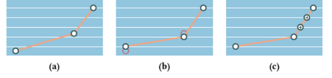
Figure 5: Layer/anchor snapping process. (a) Cross-sectional view of input anchor points \circ and fiber path \text{—} , against layers \text{—} (layer thickness exaggerated). (b) Anchor points snapped to the nearest layer boundary. (c) New anchor points added where fiber crosses layers without anchor points defined.
