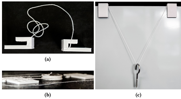
Figure 25: Embedded fiber can enable fabricating objects larger than the printer's build volume. (a) A hook printed to hang from a door (c) can be created by wrapping extra fiber around a temporary structure on the print bed (b).
