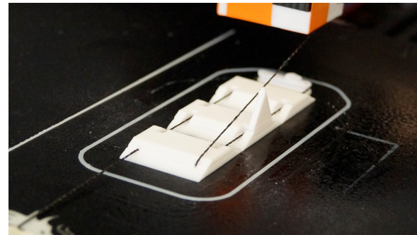
Figure 20: Self-assembling box on the build plate, with an off-object anchor visible just behind the object.
