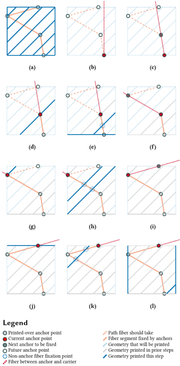
Figure 4: A step-by-step example of Rhapsody's routing algorithm operating on a single layer of an object. (a) A preview of the finished layer. (b) The initial state of the layer and fiber. (c) The fiber rotates to cross the next anchor point. (d) The fiber is anchored via a print over operation. (e) Geometry which does not interfere with the fiber's upcoming paths is printed, including further fixations. (f) The fiber rotates to cross the next anchor point. (g) The fiber is anchored via a print over operation. (h) Geometry which does not interfere with the fiber's upcoming paths is printed, including further fixations. Note the line of geometry closest to the anchor point which, if printed at this stage, would prevent the fiber being fixed by that line. (i) The fiber rotates to cross the next anchor point. (j) The fiber is anchored via a print over operation. (k) Now the line of geometry can be printed over both segments of fiber it crosses. (l) All remaining unprinted geometry is printed.
