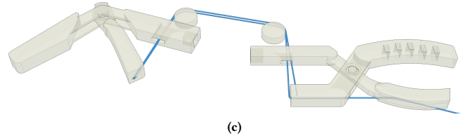
Figure 23: Our grabber device was printed as two plastic parts connected by thread and which, after printing, are rigidly connected using an inserted stick.
