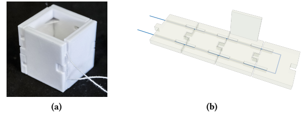
Figure 18: (a) Box printed flat, assembled by pulling threads. (b) Transparent view showing internal thread routing.
