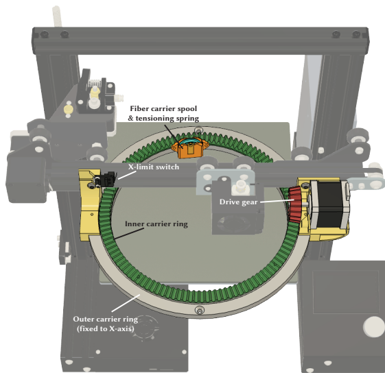
Figure 6: Detail view of Rhapso implementation.
