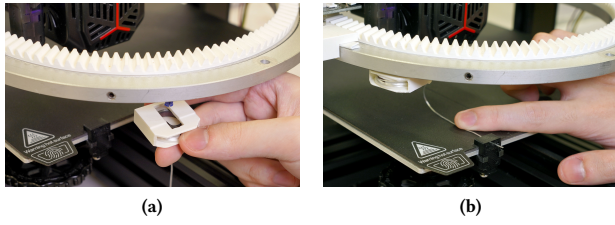
Figure 11: (a) We attach a fiber spool with a rotational spring inside to the ring. (b) Our bed anchor attaches one end of the fiber to a consistent location on the print bed.
