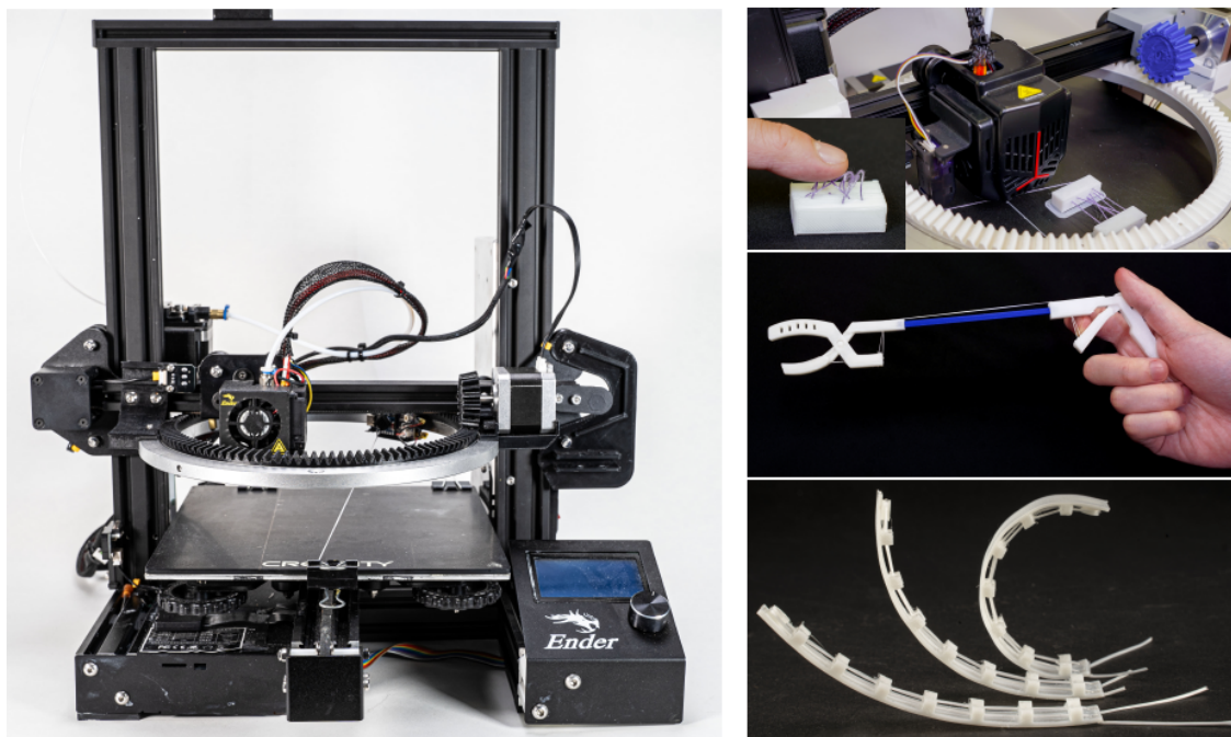
Figure 1: Rhapso allows embedding various types of fibers into 3D prints to enable quick fabrication of multifunctional objects. Left: Rhapso hardware made by modifying a consumer grade 3D printer. An added fiber spool is moved along the attached ring. Right: Objects created by Rhapso. Top: Hairy object. A cotton fiber is embedded between two cuboids and creates hairy texture. Middle: Grabber. The white elastic thread transfers users' pinch to the extended grabber. Bottom: Test of tension control system. The same 3D design can result in different shapes by controlling the tension of the elastic fiber during printing.
