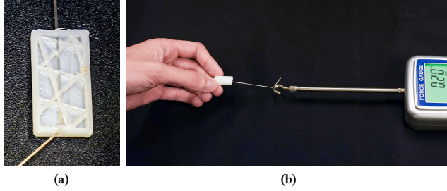
Figure 14: Adhesion test object, shown with spandex fiber. (a) Print paused one layer above fiber-embedding layer, showing layer lines acting as additional anchors. (b) Testing setup.
