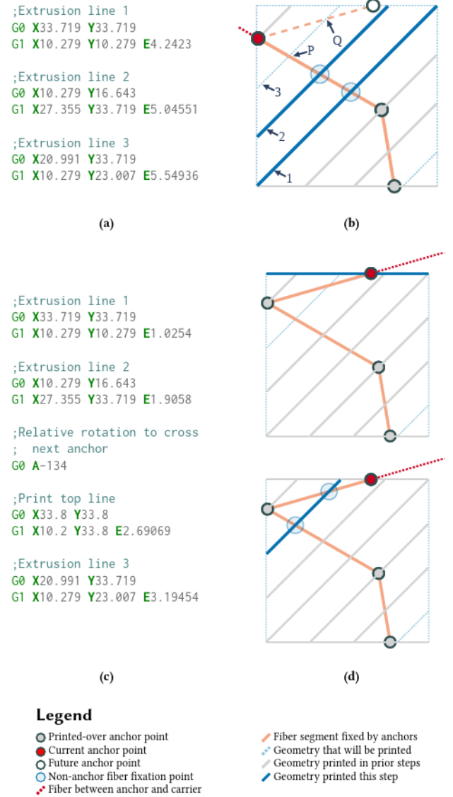
Figure 8: (a) G-code from slicer that would print lines 1–3 of (b) in order. (c) G-code modified by Rhapsody to print lines 1 and 2 (b), rotate the fiber and fix it at the anchor (d, top), then print line 3 (d, bottom).
