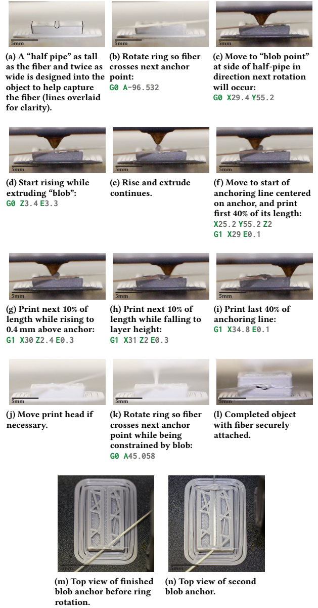
Figure 13: “Blob” anchoring procedure for stronger anchor/-plastic adhesion.
