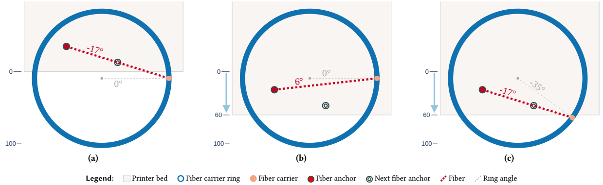
Figure 9: On printers with an XZ-head configuration, the print bed moves relative to the ring, changing the fiber angle. (a) The initial printer state, viewed top-down. (b) If the bed moves and the ring does not, the fiber angle changes. (c) Rhapso synchronizes ring moves to bed moves to keep a constant fiber angle.
