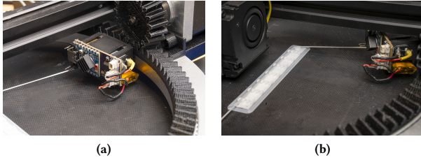
Figure 26: Automatic tensioning feeder: (a) the automatic tensioning feeder controlled via Wi-Fi through an ESP32 module, (b) the feeder applying tension between anchor points. Figure 1d shows three flexible samples printed with the same geometry embedded with elastic threads elongated at different ratios achieved with controlled tensioning.
