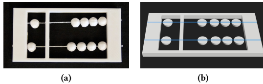
Figure 17: (a) Abacus printed with free-sliding beads. (b) Cut-away view of embedded fiber design.
