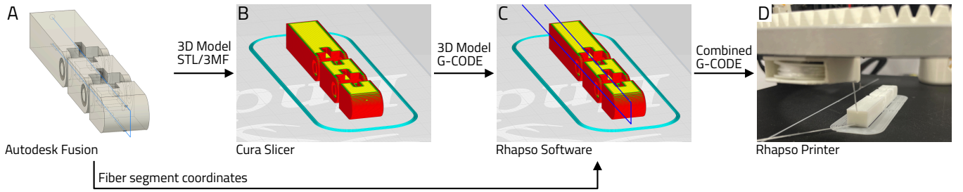
Figure 3: Walkthrough of fabricating robot finger in 6.6. (A) Users draw a 3D (blue) line that will be embedded in the 3D model and export the line and 3D model separately. (B) The 3D model is sliced and converted to G-code. (C) Our custom software generates G-code for line embedding and combines it with 3D model G-code. Note that the image is conceptual; our software visualizes the process on a 2D plane as in Figure 4(a). (D) Our modified 3D printer embeds an elastic fiber in the finger as designed.
