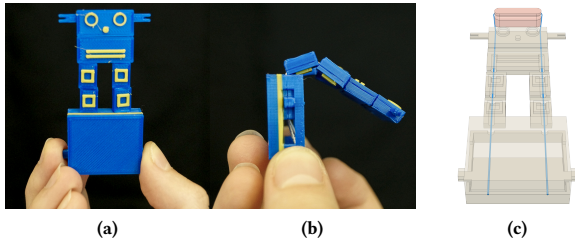
Figure 16: Robot puppet with embedded pre-tensioned elastic fiber. (a) Base pulled down to keep fiber tensed. (b) Base released to allow fiber to relax. (c) Fiber route through robot.
