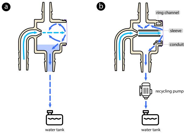
Figure 6: (a) Water accumulation, along with internal turbulence, is observed when the chamber opening is sealed with a membrane while the chamber outlet is directly connected to the water tank. (b) Connecting chamber outlet to a recycling pump, along with incorporating measures such as a protective sleeve, ring channel, and conduit, can enhance the efficiency of water egress.
