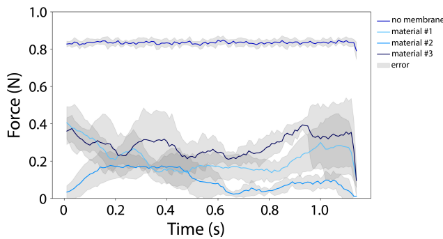
Figure 5: Force measurement results: The blue-tinted curves represent the force measurements for both the baseline and each membrane material; The grey-shaded area indicates the standard deviation of the force measurements at each timestamp.
