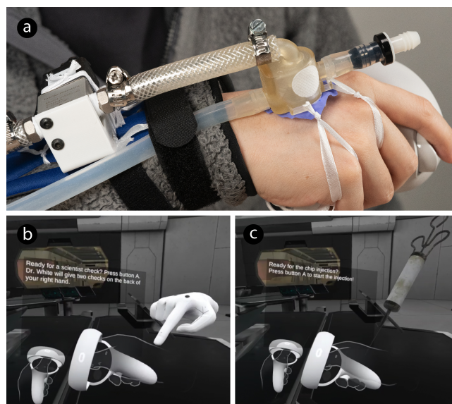
Figure 1: (a) The JetUnit offers force feedback over a wide range of perceived force intensities and pulsing frequencies. A single wearable JetUnit can render interactions ranging from (b) a gentle touch to (c) a progressively accelerating injection.
