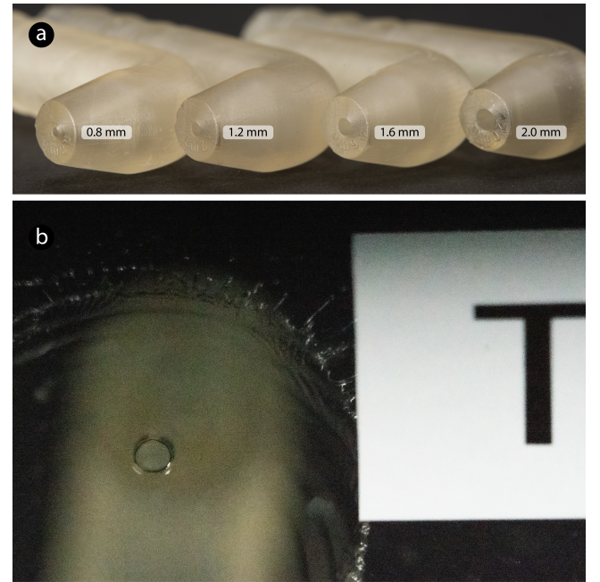
Figure 9: (a) A set of nozzle prototypes, ranging in size from 0.8 mm to 2.0 mm, is used to measure the actual contact area of water jets. (b) The set of nozzle prototypes was positioned 25 mm away from a transparent acrylic board, onto which a letter 'T' was affixed for calibration. The horizontal line of the letter measured 4.7 mm in length, and the vertical line was 4.9 mm long. Water jets were then activated, and photographs were taken. The diameter of the actual contact area can be determined through pixel-to-actual length conversion.
