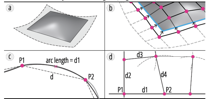
Figure 15. Modifications to Chebyshev Net Algorithm. (a) Surface extension, (b) edge trimming, (c) line-to-arc edge conversions (edge length changes from d to d1 ) in step 1; (d) Variable distance meshing in step 2.
