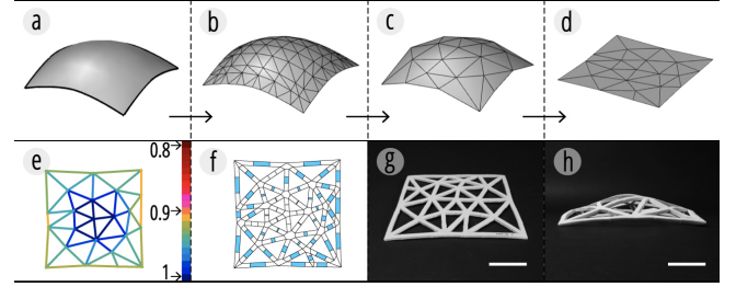
Figure 6. Shrinkage-based flattening pipeline overview. (a) Target surface S ; (b) Meshed S ; (c) Simplified mesh M ; (d) flattened Pattern M_f ; (e) length distortion; (f) actuator assignments; (g) fabricated artifact; (h) triggered artifact. (Scale bar: 5 cm)
